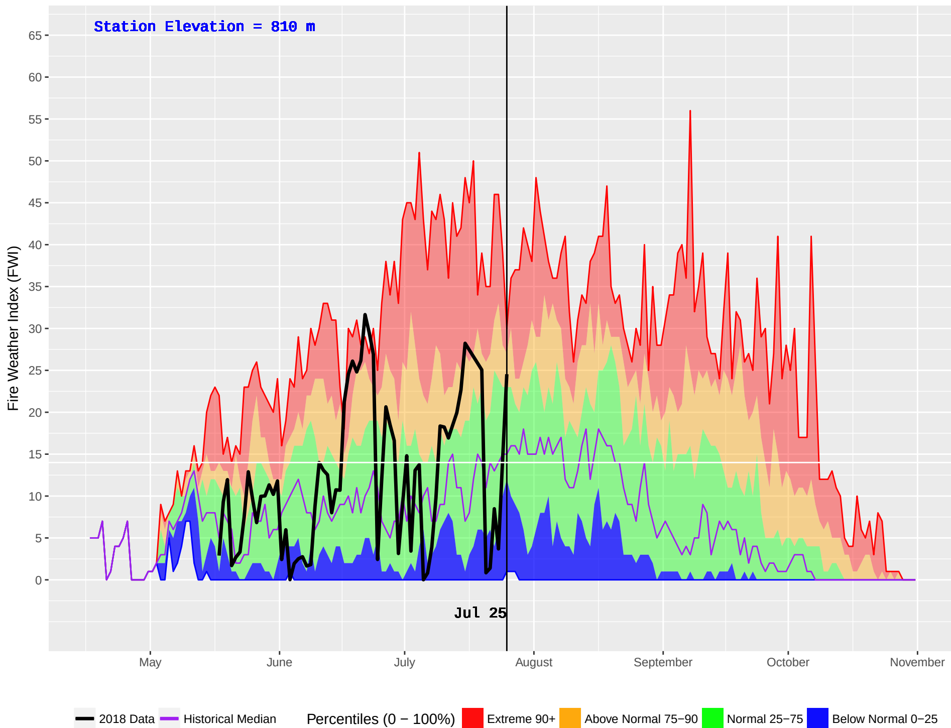
MCBRIDE LAKE (180) : Historical (1990–2016) and Current (2018) Noon Fire Weather Index (FWI)
