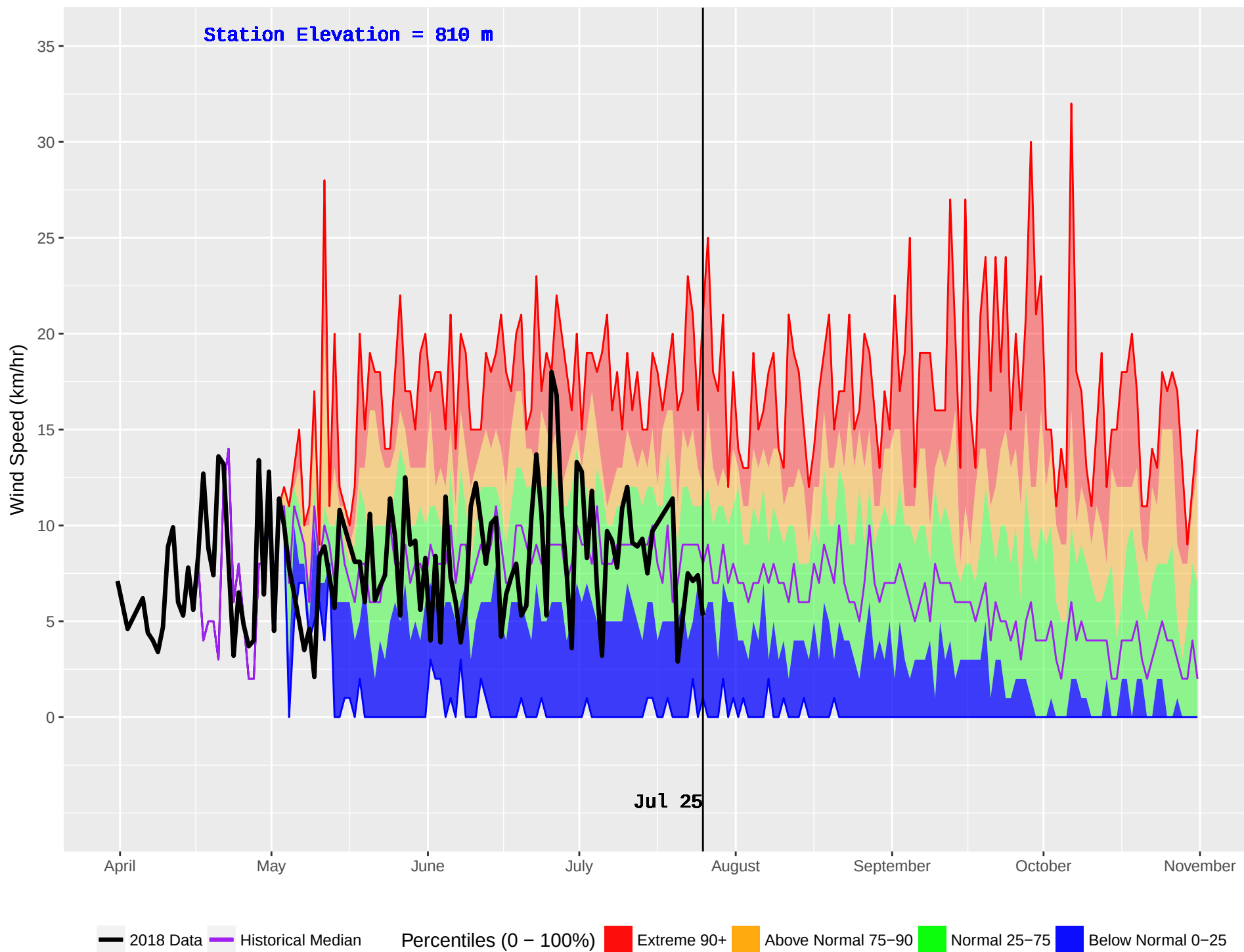
MCBRIDE LAKE (180) : Historical (1990–2016) and Current (2018) Noon Wind Speed
