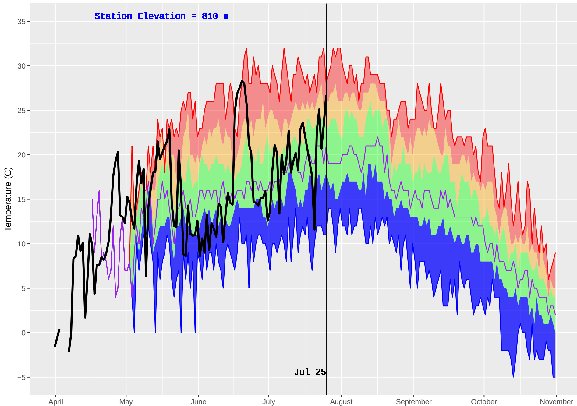
MCBRIDE LAKE (180) : Historical (1990–2016) and Current (2018) Noon Temperature
