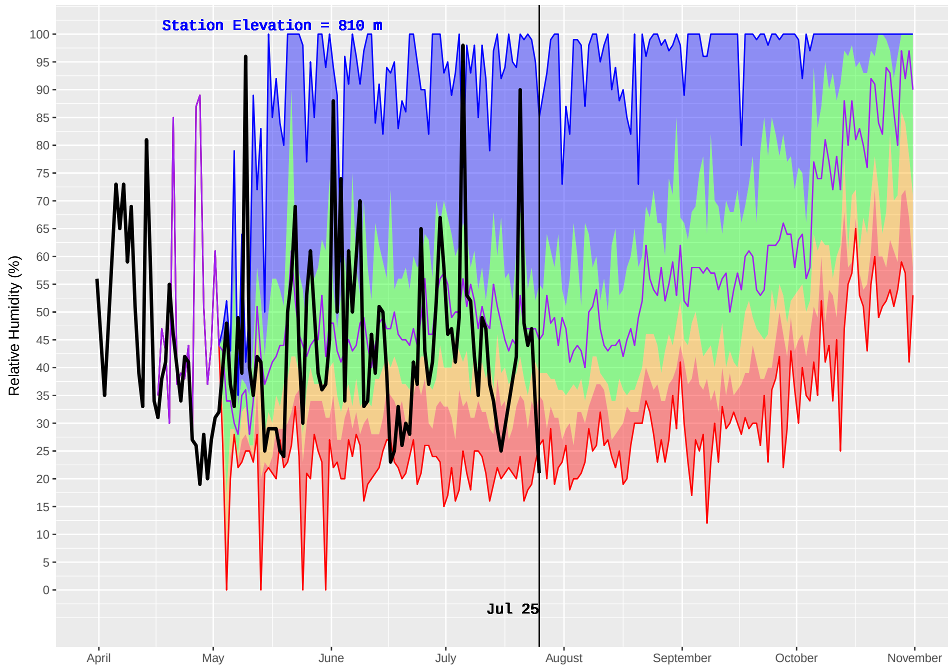
MCBRIDE LAKE (180) : Historical (1990–2016) and Current (2018) Noon Relative Humidity
