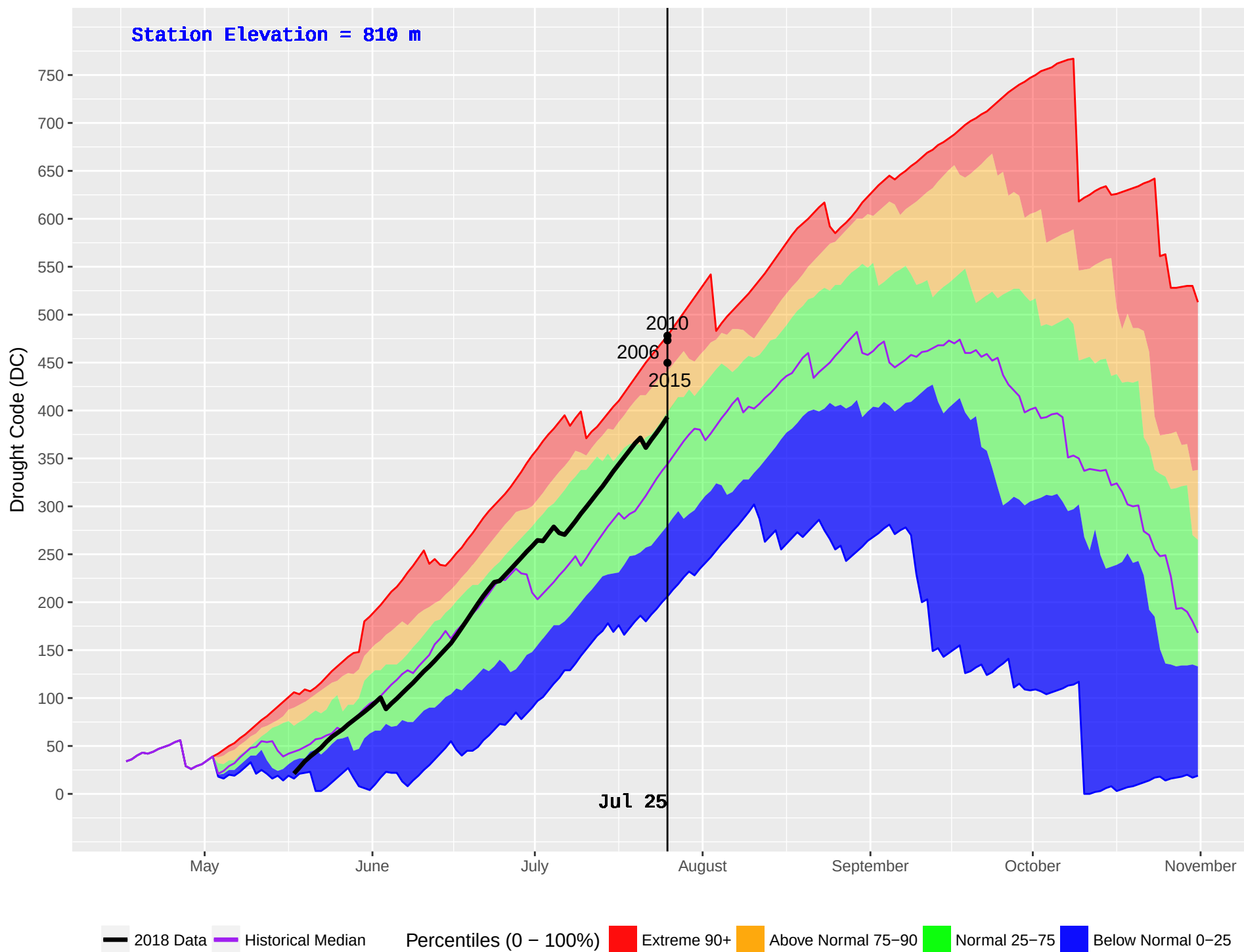
MCBRIDE LAKE (180) : Historical (1990–2016) and Current (2018) Noon Drought Code (DC)
