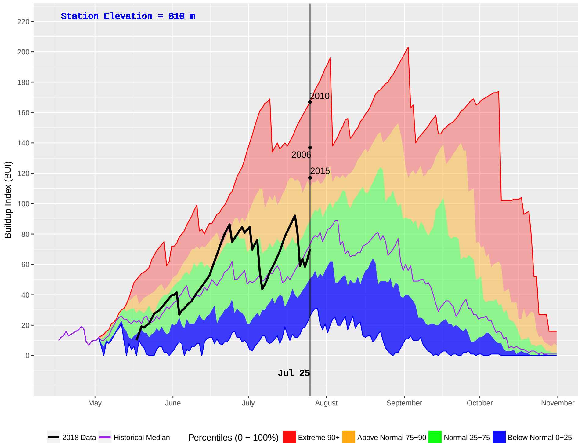
MCBRIDE LAKE (180) : Historical (1990–2016) and Current (2018) Noon Buildup Index (BUI)
