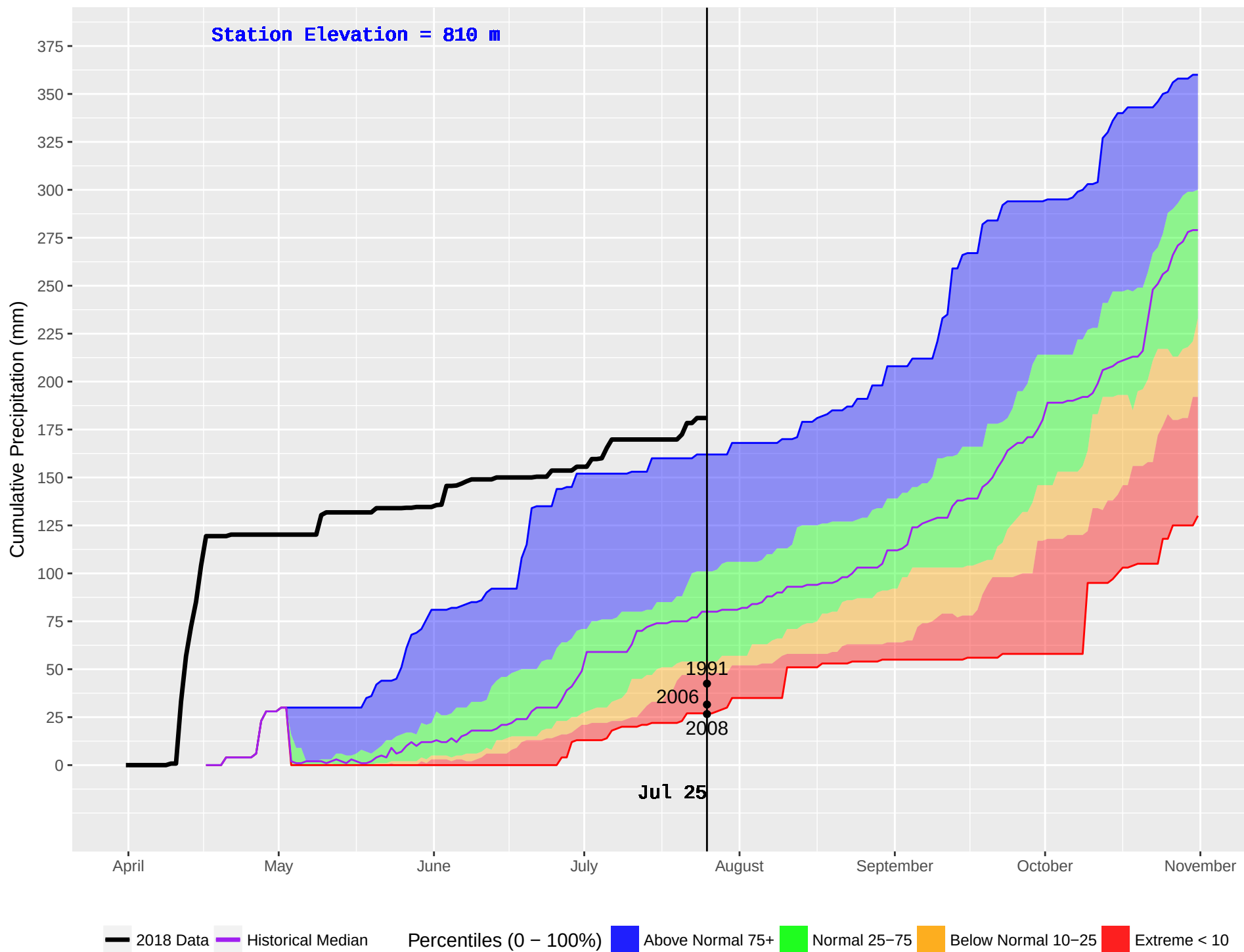
MCBRIDE LAKE (180) : Historical (1990–2016) and Current (2018) Noon Cumulative Precipitation
